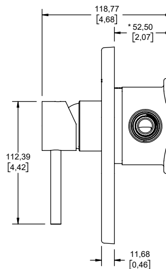
VISTA LATERAL SIDE VIEW
